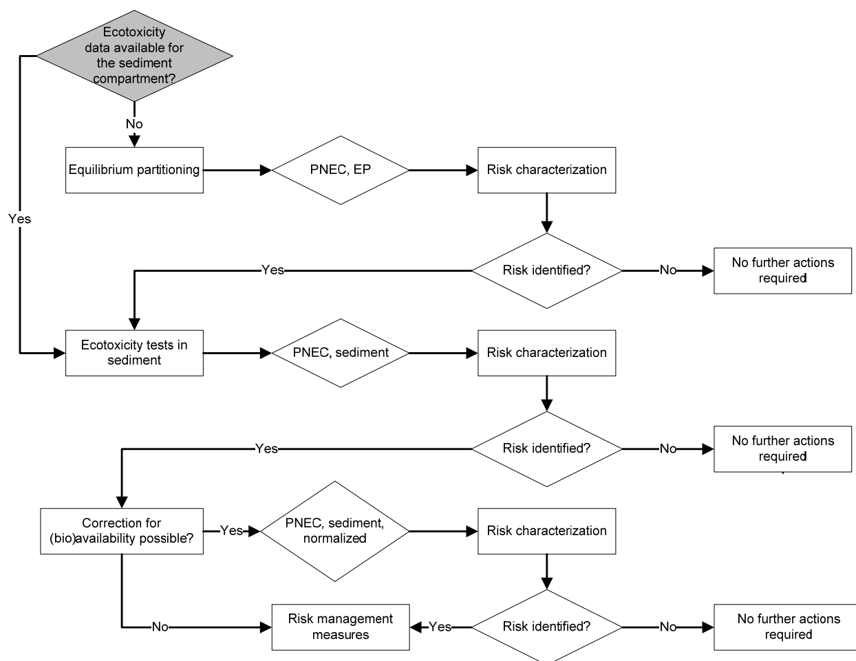
Figure 12: General framework for sediment risk characterisation.
