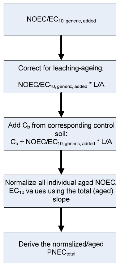
Figure 15: Framework for the calculation of a site specific PNEC soil.
